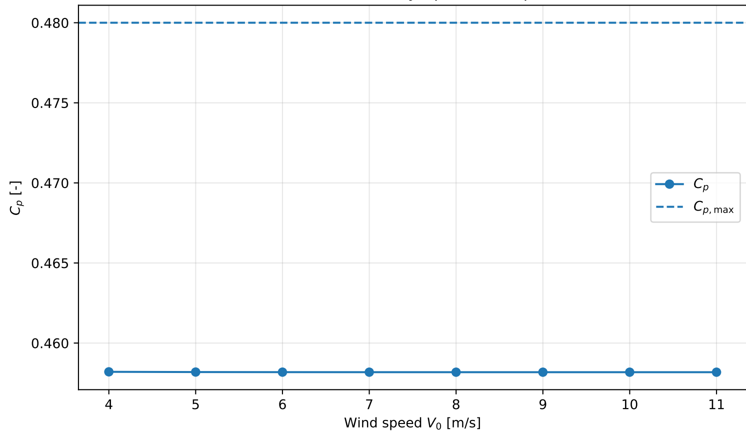
Below-rated steady C_p vs wind speed
